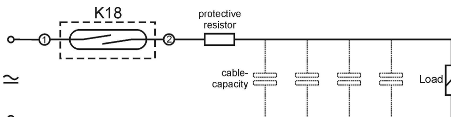
Fig. 9 Protective circuit for current limitation
