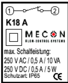
Fig. 7 Contact K 18 A
