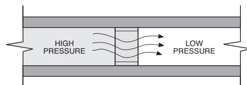
Flow Restrictor: Gas moves uniformly through porous metal element with minimal friction due to viscosity.
